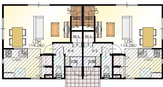
1F
